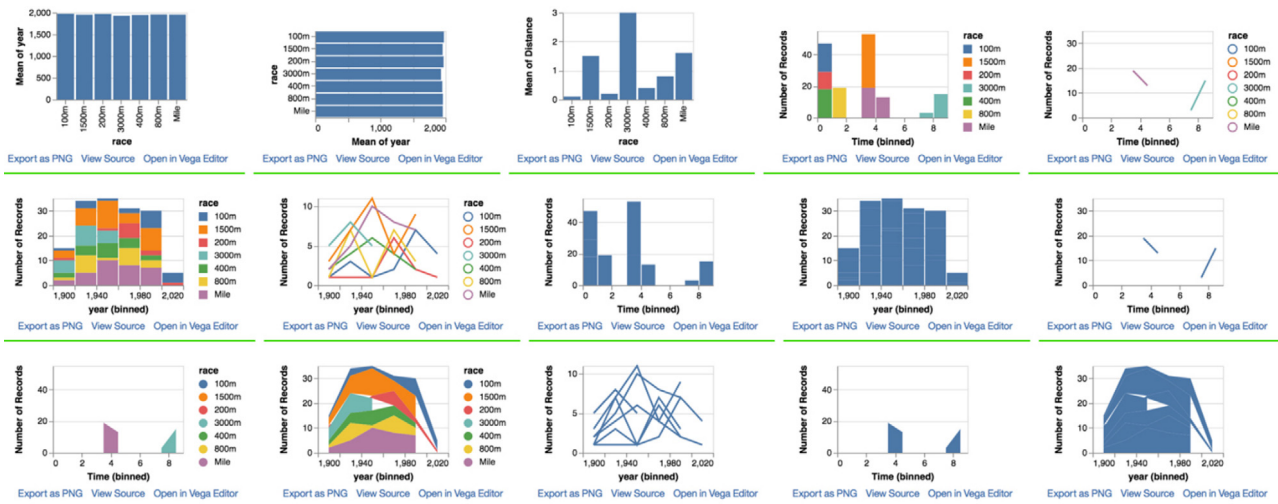
Fig. 6. Visualization alternatives generated by Data2vis.
