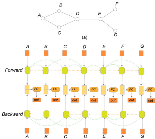
Fig. 9. An illustration of graph-LSTM-based model architecture in DeepDrawing (Wang et al., 2019a).
