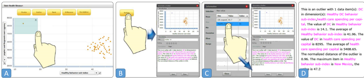
Fig. 15. A scenario where a user annotates an outlier using Touch2Annotate , which involves three steps: (A) selection of the outliers by drawing a rectangular boundary to; (B) generation of an annotation; (C) dragging of items into the annotation; (D) final annotation.
