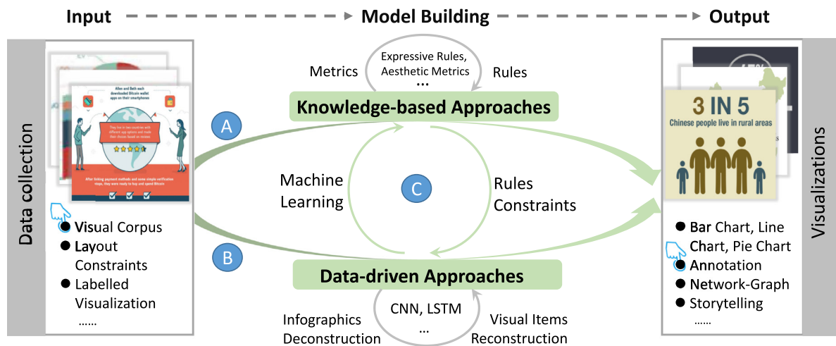
Fig. 2. Three paths of automatic infographics and visualizations. Existing works are divided into three categories: (A) knowledge-based approaches; (B) data-driven approaches; and (C) hybrid approaches.
