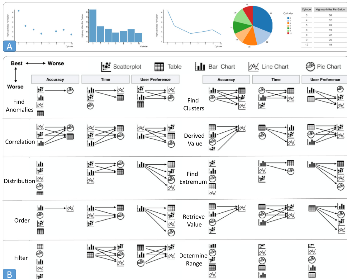
Fig. 5. (A) General types of visualizations used in Saket et al. (2018), such as scatterplot, bar chart, line chart, pie chart, and table. (B) Correlations between visualization types across tasks and performance metrics.
