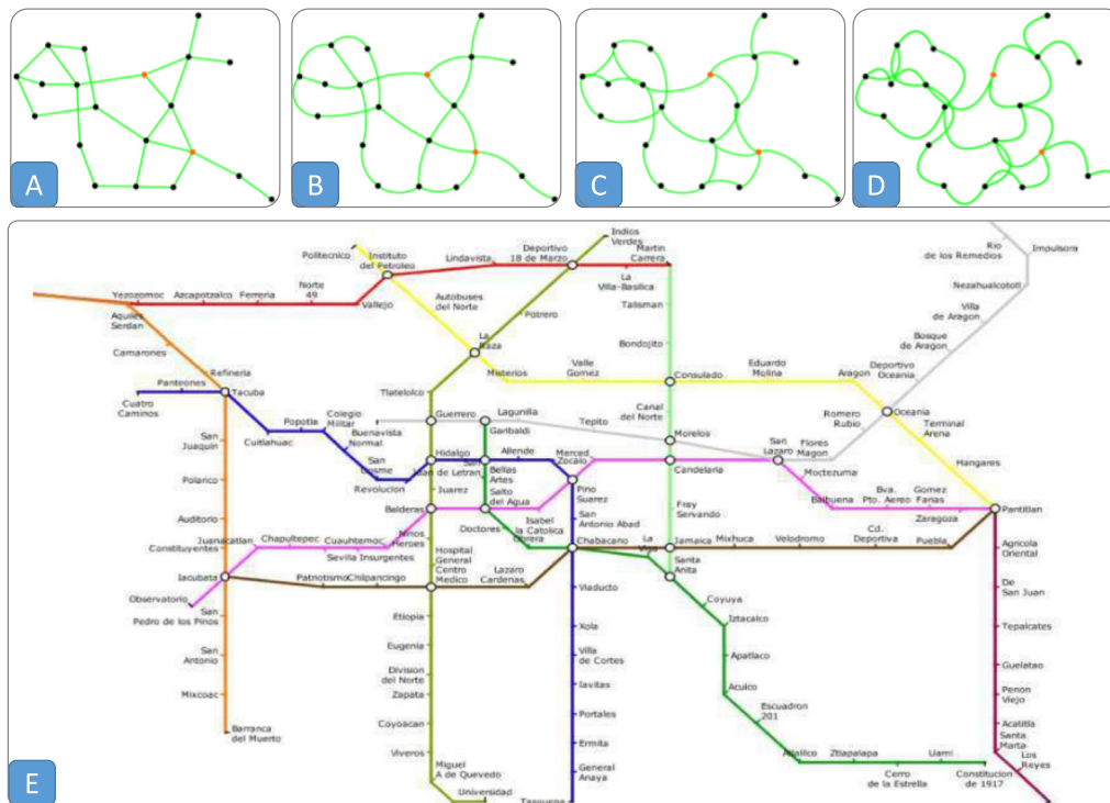
Fig. 18. (A–D) Examples of edge types used in the cured edge study. (A) Straight edge, (B) Lombardi layout, (C) Slightly curved edge, (D) Heavily curved edge. (E) Visualization of automatic metro map layout using multicriteria optimization.
