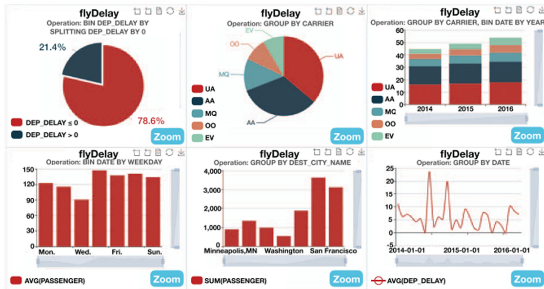
Fig. 19. Charts are automatically generated by DeepEye.
